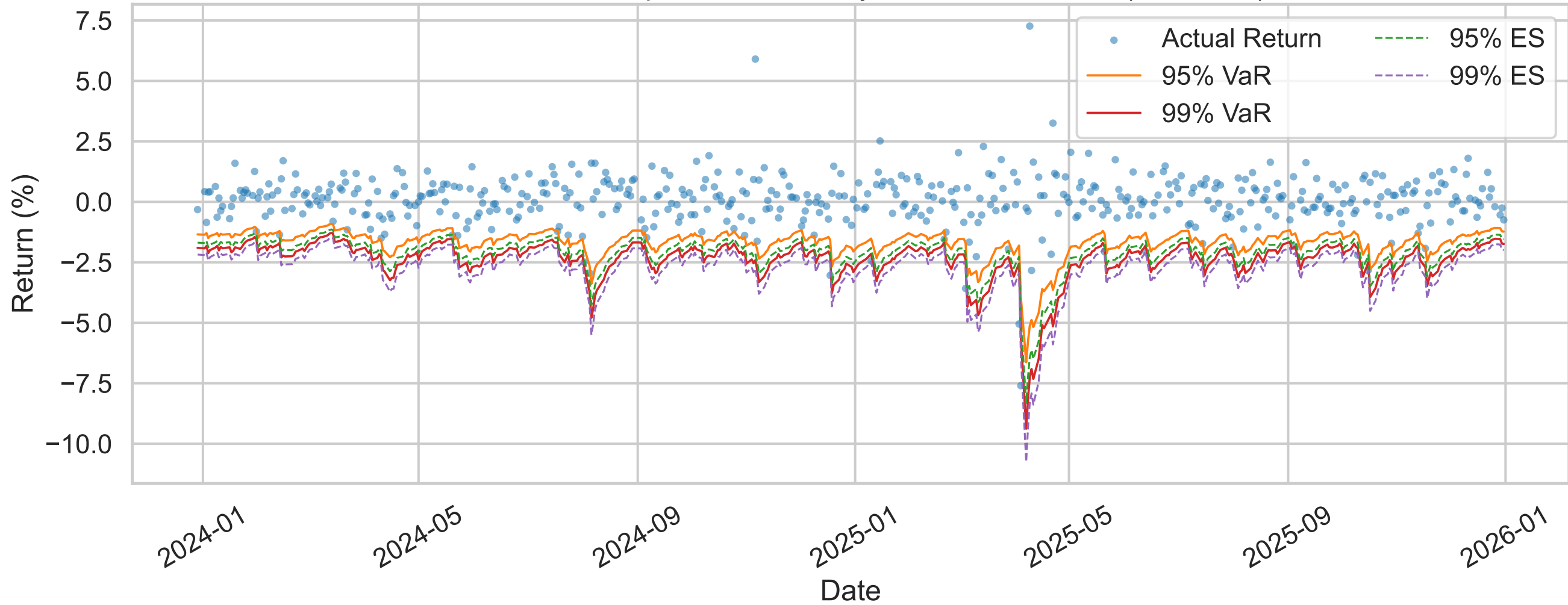
XLF Out-of-Sample Returns vs Dynamic VaR and ES (EGARCH)
